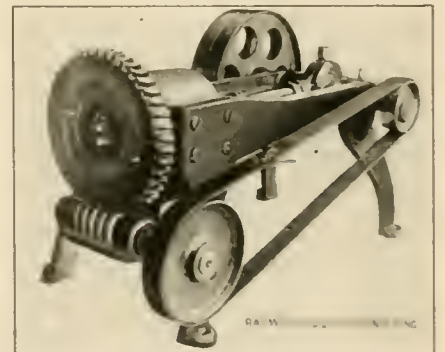
ANOTHER VIEW OF MACHINE FOR GRINDING PACKING RING INTO TRIPLE VALVE.
